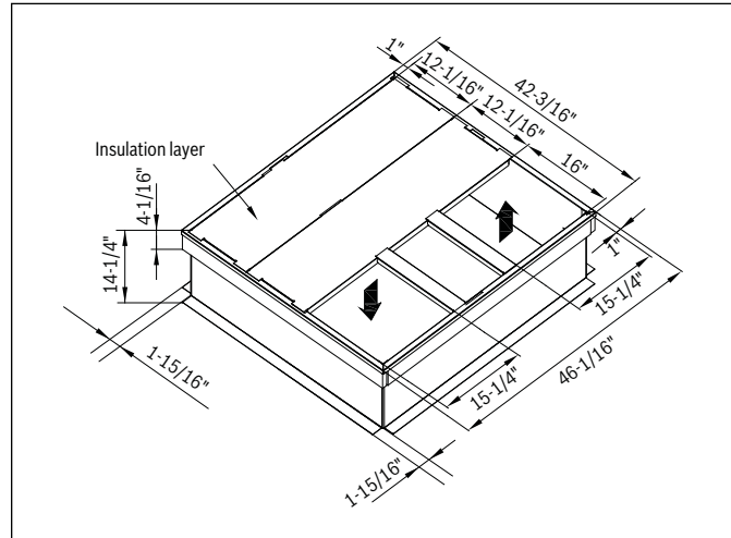
Figure 6 Roof Curb Dimensions
