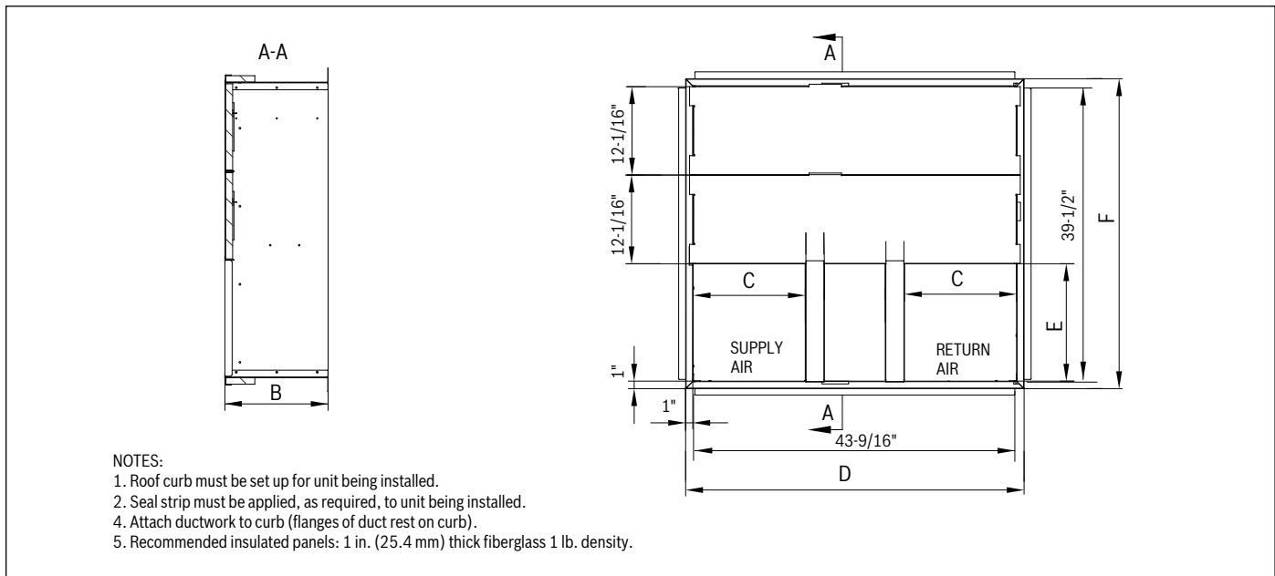
Figure 5 Roof Curb Details
